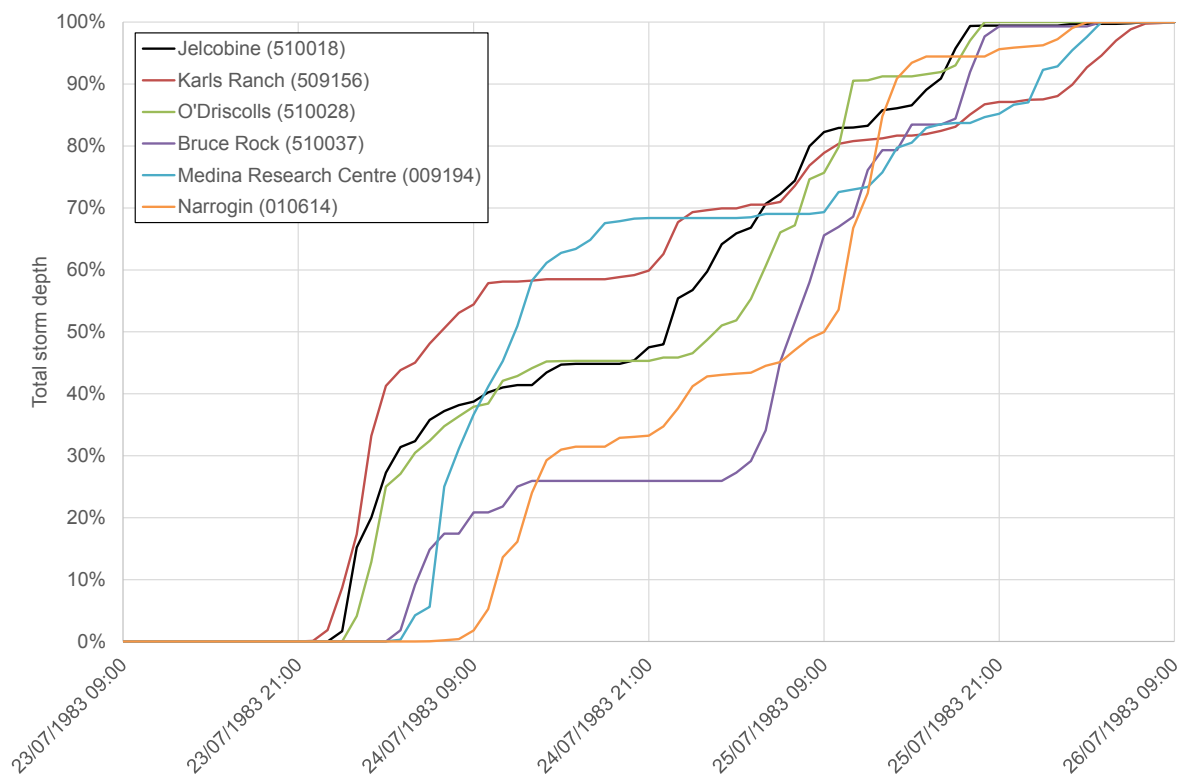
■ Figure 6-21: July 1983 pluviograph data
