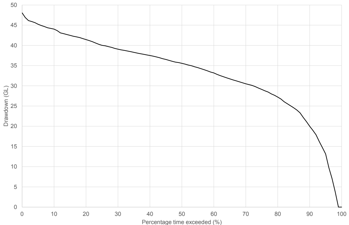
■ Figure 8-16: Mundaring Dam exceedance curve of storage below FSL 1954-2015
