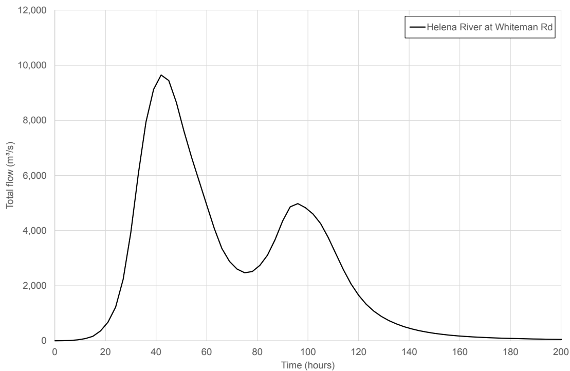
■ Figure 10-6: Indicative PMF hydrograph at Whiteman Road
