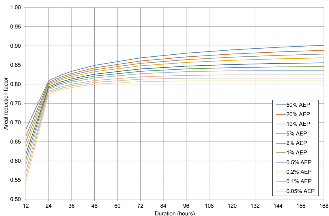
■ Figure 8-1: Lower catchment areal reduction factors
