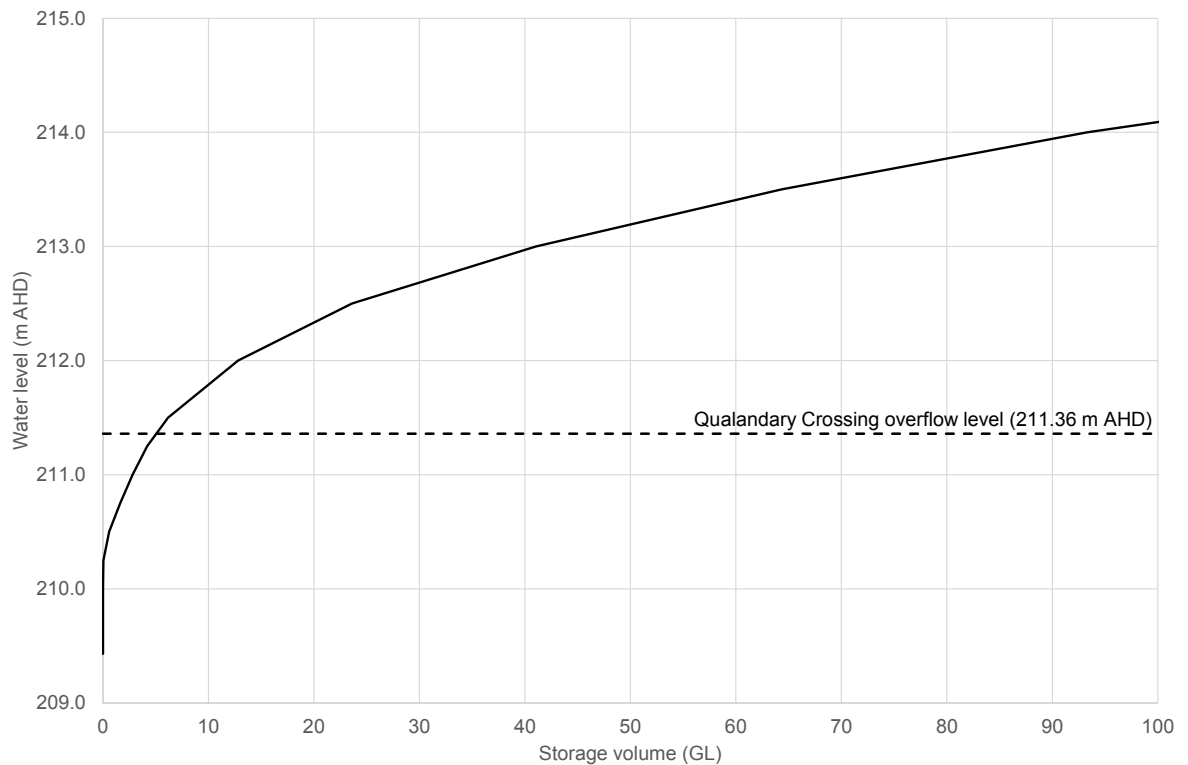
■ Figure 5-6: Yenyenning Lakes stage-storage relationship
