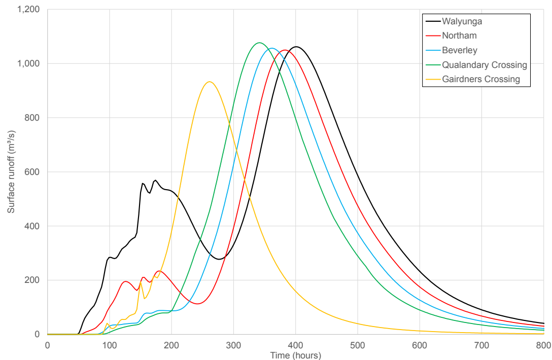
■ Figure 10-2: Typical hydrographs for 1% AEP flood – complete catchment (note baseflow not included)
